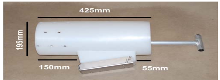
LA8000 — Large round transom mounted removable burley bucket including chomper.
