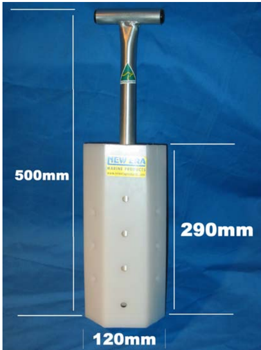
LA8010 — Small transom mounted burley bucket including chomper.
