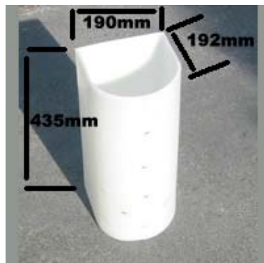
LA8005 - "D" shaped burley bucket fixed including chomper.
